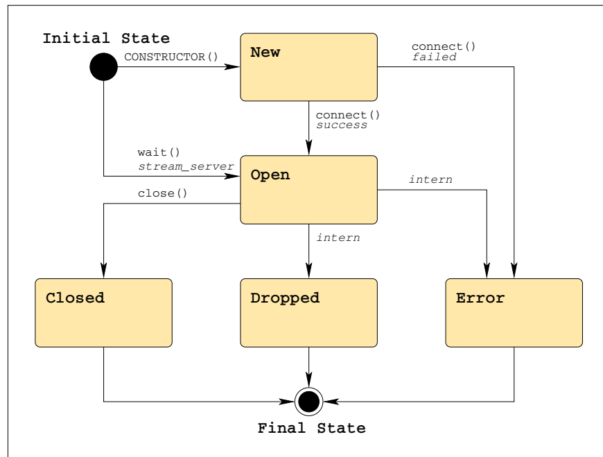
Figure 6: The SAGA stream state model (See Figure 1 for a legend).
